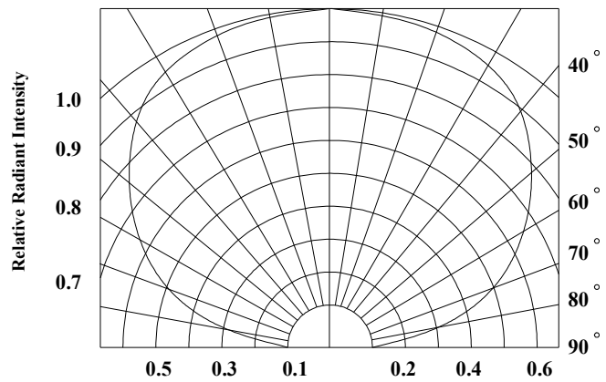
Radiation diagram
