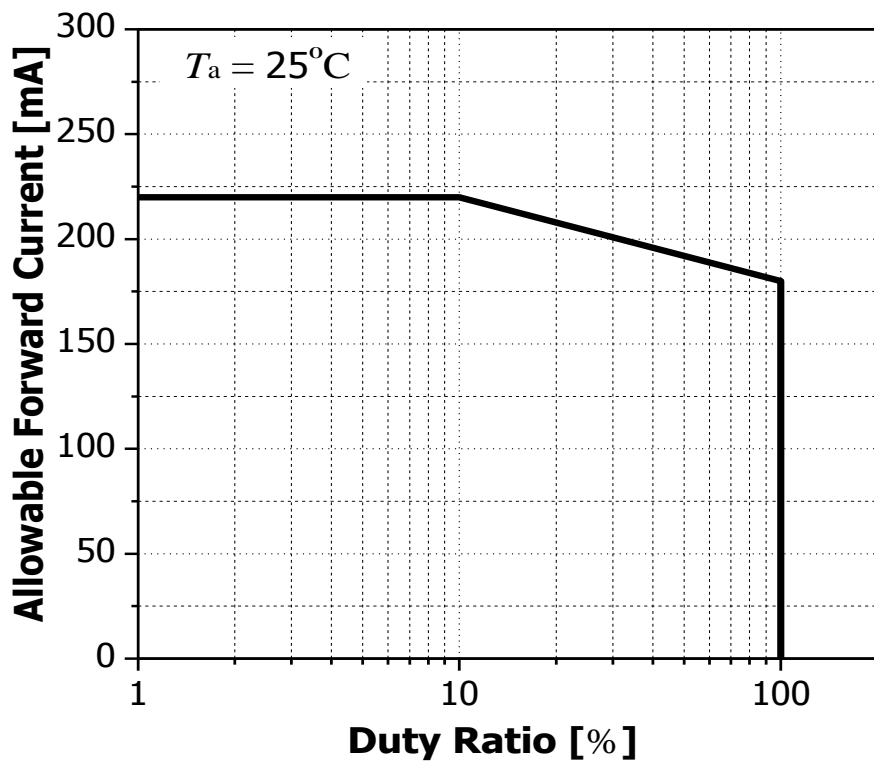
Fig 9. Allowable Forward Current vs. Duty Ratio, T_a = 25^\circ\text{C} , 1kHz
