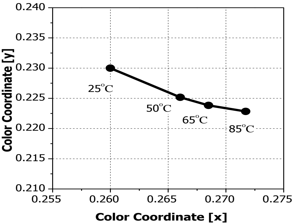
Fig 6. Color Coordinate vs. Ambient Temperature, I_F = 120\text{mA}
