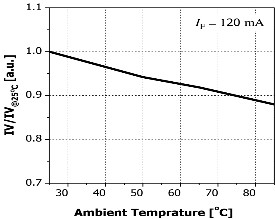
Fig 8. Relative Luminosity vs. Ambient Temperature, I_F=120\text{mA}
