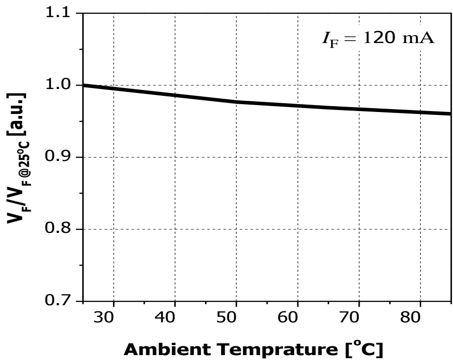
Fig 7. Forward Voltage vs. Ambient Temperature, I_F=120\text{mA}
